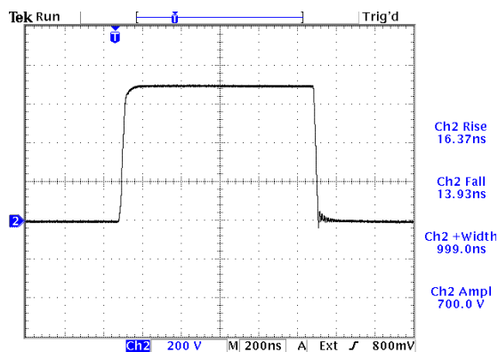
A 700V, 1us pulse from model AVR-7B-B
