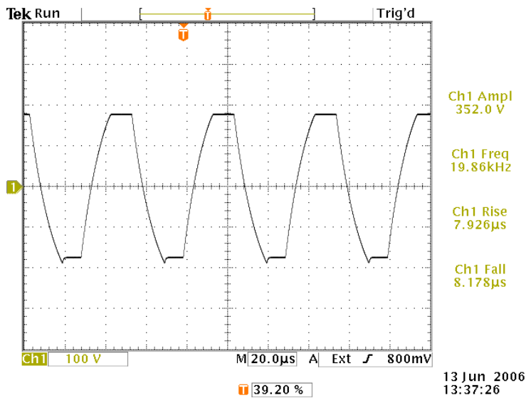
Square wave output into a load consisting of 1.2 kΩ and 10000 pF in parallel. Amplitude set to 180V. 20 kHz, 20 us / div, 100 V/div.
