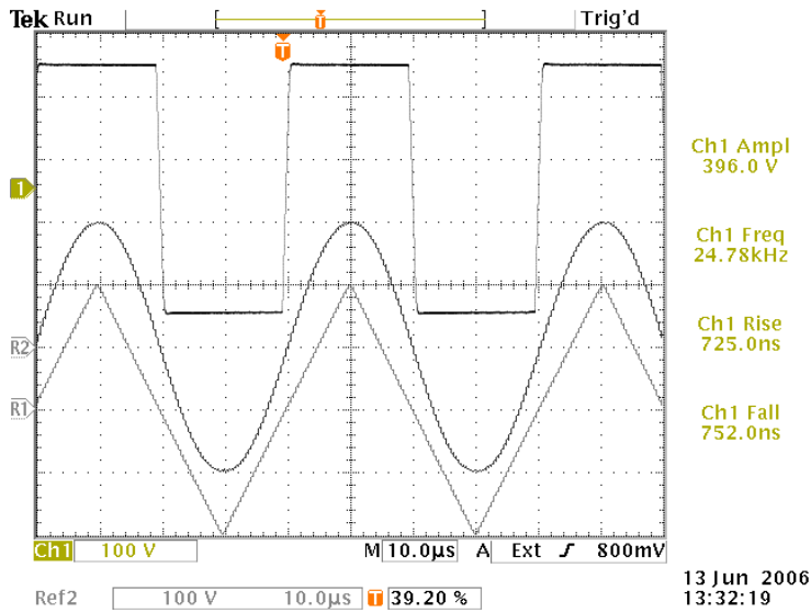
Square, Sine, and Triangle outputs into a 1.2 kΩ load at maximum amplitude. 25 kHz. 100 V/div, 10 us/div.
