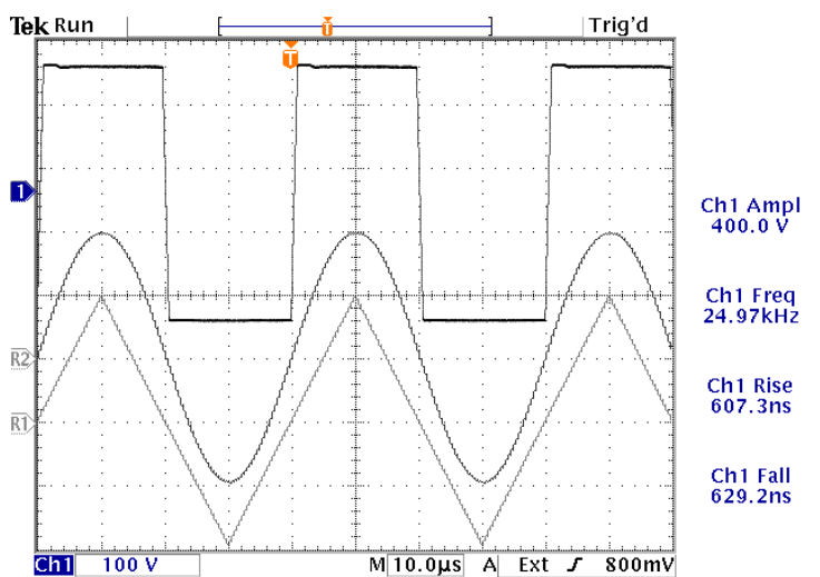
Square, Sine, and Triangle outputs into a 1.2 kΩ load at maximum amplitude. 25 kHz. 100 V/div, 10 us/div.
