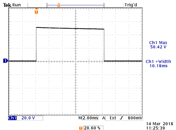
10 Hz, 10 ms, +50V, into 50Ω. 20V/div, 2 ms/div.
