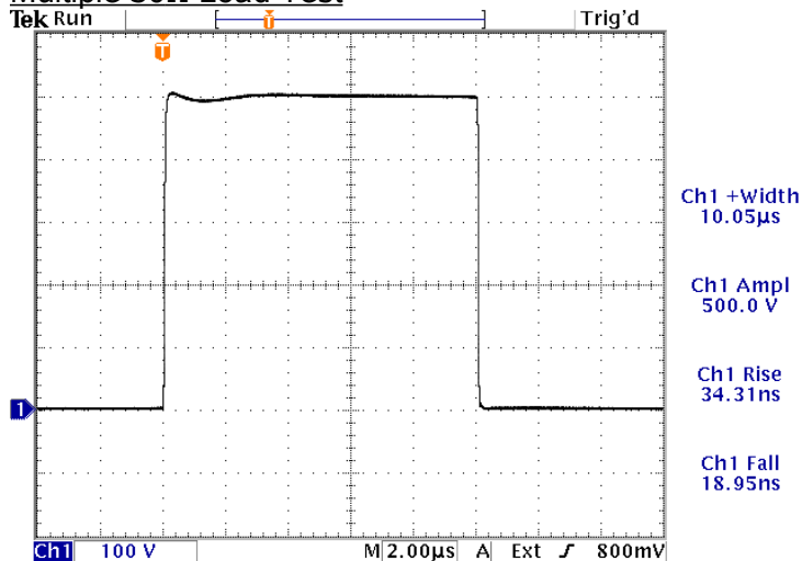
Multiple 50Ω Load Test
