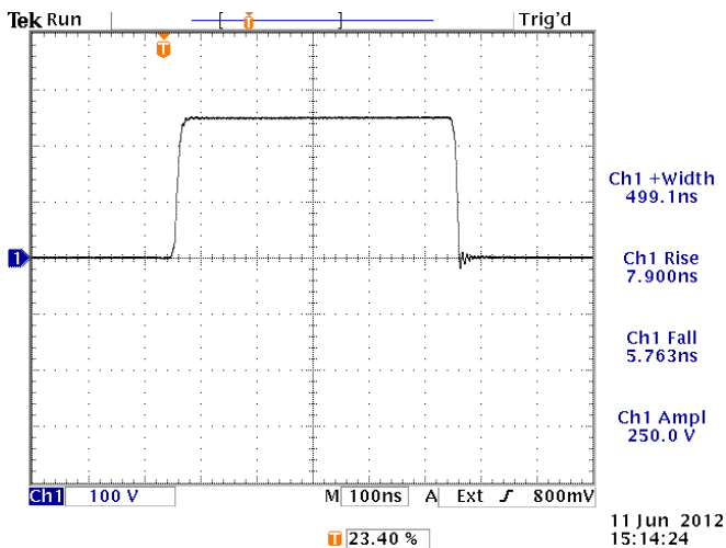
10 kHz, 500 ns, +250V into a 50Ω load. 100 V/div, 100 ns/div.
