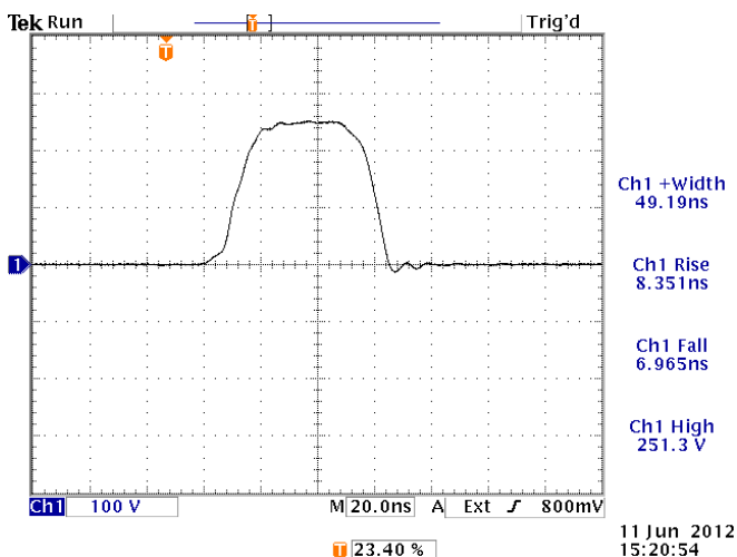
100 kHz, 50 ns, +250V into a 50Ω load. 100 V/div, 20 ns/div.
