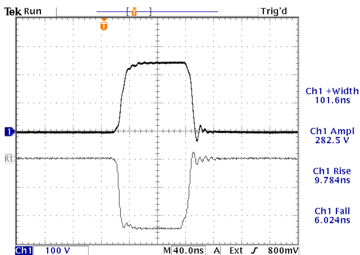
7 Sep 2012 09:42:57 Ref1 100 V 40.0ns 31.00 % 100 kHz, 100 ns, +250V and -250V into a 50Ω load. 100 V/div, 40 ns/div.
