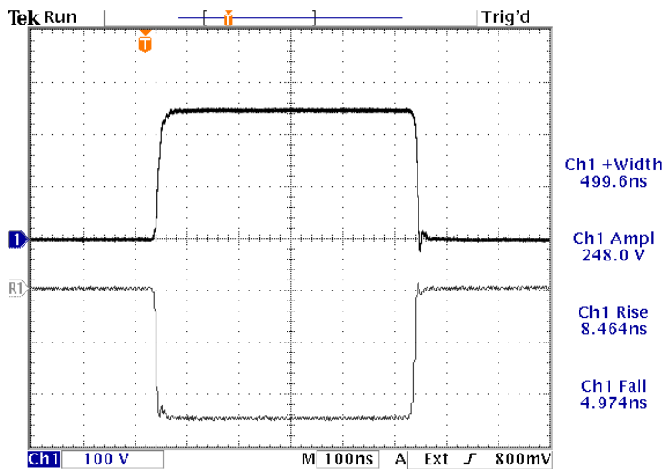
7 Sep 2012 09:43:36 Ref1 100 V 100ns 22.00 % 10 kHz, 500 ns, +250V and -250V into a 50Ω load. 100 V/div, 40 ns/div.
