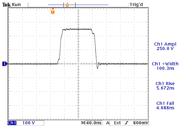
100 kHz, 100 ns, +250V, into a 50Ω load. 100 V/div, 40 ns/div. 20 Sep 2013 10:39:10 31.80 %
