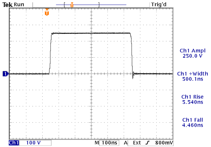
10 kHz, 500 ns, +250V, into a 50Ω load. 100 V/div, 100 ns/div. 20 Sep 2013 10:37:44 22.80 %
