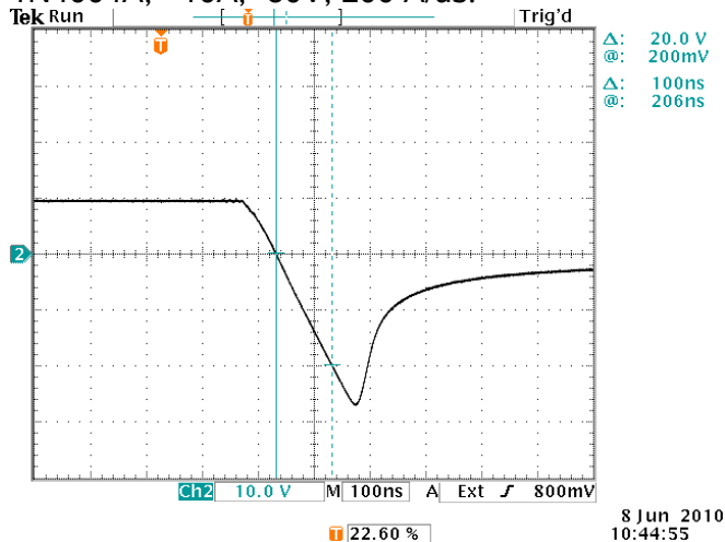
1N4004A, +10A, -80V, 200 A/us.
