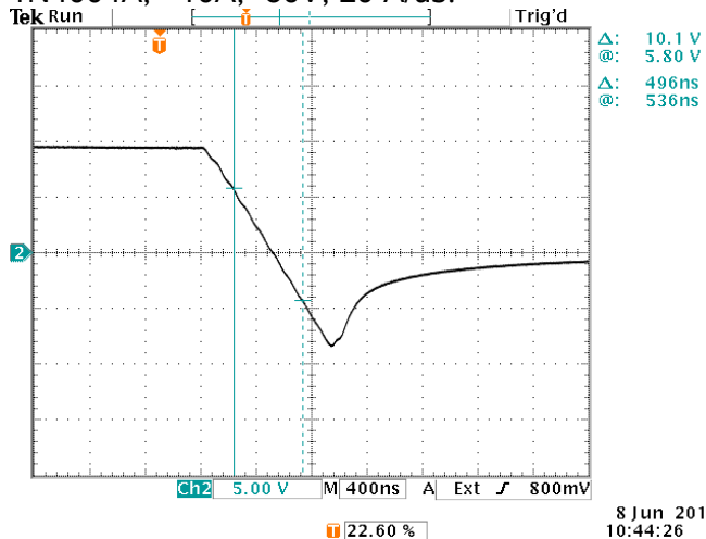
1N4004A, +10A, -80V, 20 A/us.
