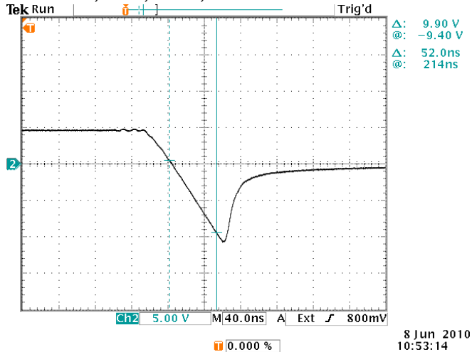
1N4937A, +5A, -80V, 200 A/us.
