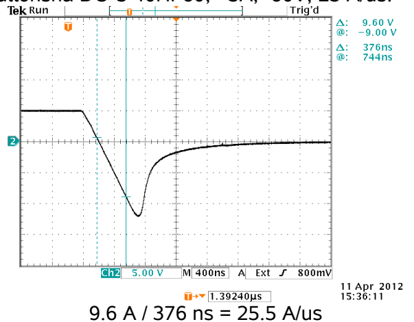
Ruttonsha DO-5 40HF80, +5A, -80V, 25 A/us.
