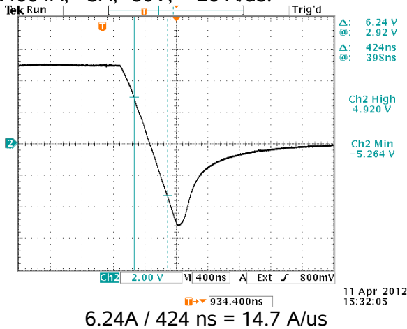
1N4004A, +5A, -80V, < 20 A/us.
