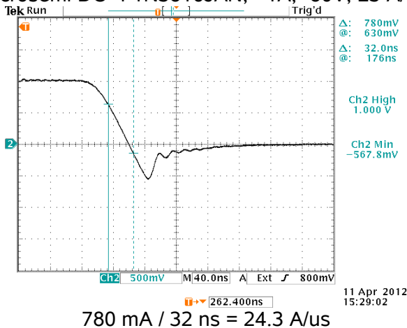
Microsemi DO-4 1N5816JAN, +1A, -80V, 25 A/us.
