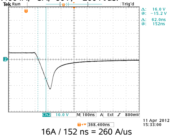
1N4004A, +5A, -80V, > 200 A/us.
