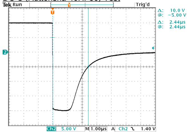
DO-5 (Ruttonsha 40HF80) Test
