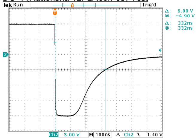
DO-4 (Ruttonsha 12FLR60/F05) Test
