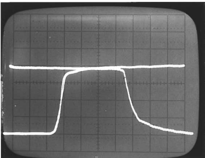
12 VOLTS/DIV, 1 NSEC/DIV
