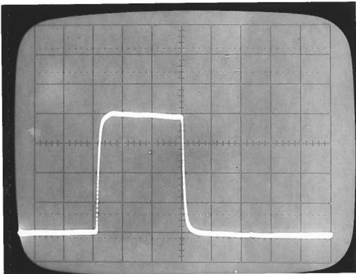
12 VOLTS/DIV, 20 NSEC/DIV
