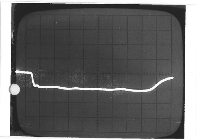
MID RANGE OUTPUT 1.0 nsec/cm
