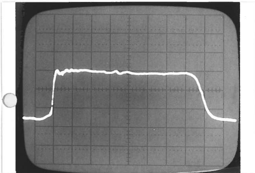
1.0 nsec / DIV ≈ 6.0 VOLTS / DIV
