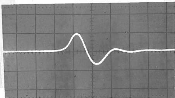
5.0 MHz PRF 10 VOLTS / DIV 0.5 NSEC / DIV
