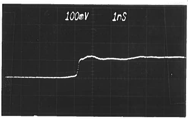
Ⓑ 60 db ATTEN (100 VOLTS/DIV) 5 KHz (RISE TIME)
