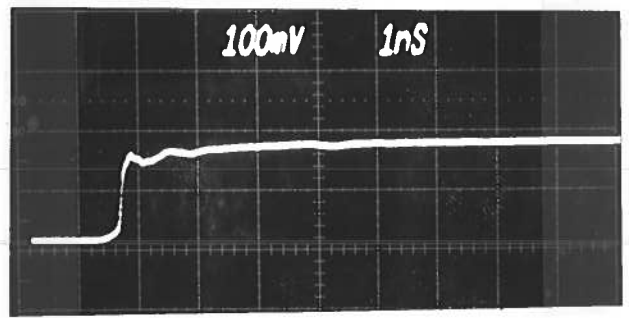
(B) 40 db ATTEN RISE TIME
