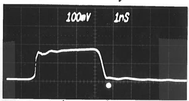
(A) 40 db ATTEN MIN PW
