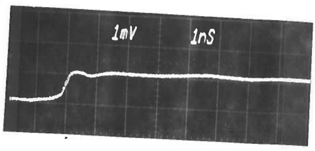
B RANGE (RISE TIME)
