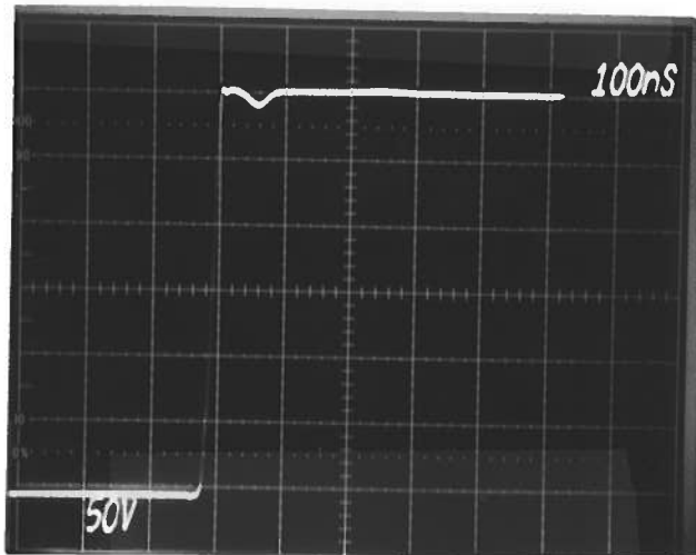
Ⓑ LOW DUTY CYCLE (RISE TIME)
