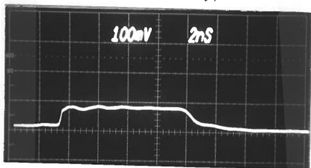
③ OUT PULSE 10 db ATTEN AS ② BUT 0.01 ufd BLOCKING CAPACITOR ON OUTPUT.
