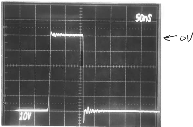
(B) AS (A) BUT 50NS/DIV
