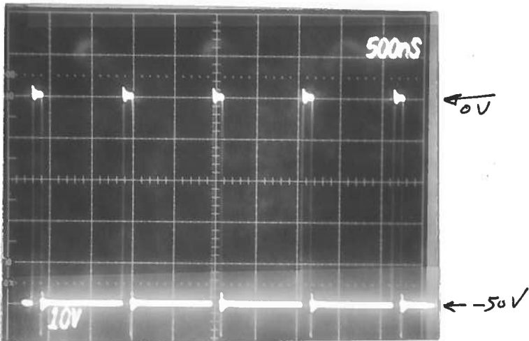
(A) Pout WITH -50V OFFSET. PRF = 1.0 MHz
