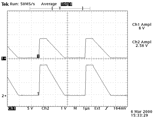
Top: AMP input, from AV-1000-C pulse generator. EXT AMPLIFY mode. 5 V/div, 1 us/div. Bottom: OUT, 0.4A into 6Ω load at end of LZ6 transmission line. 1 V/div, 1 us/div
