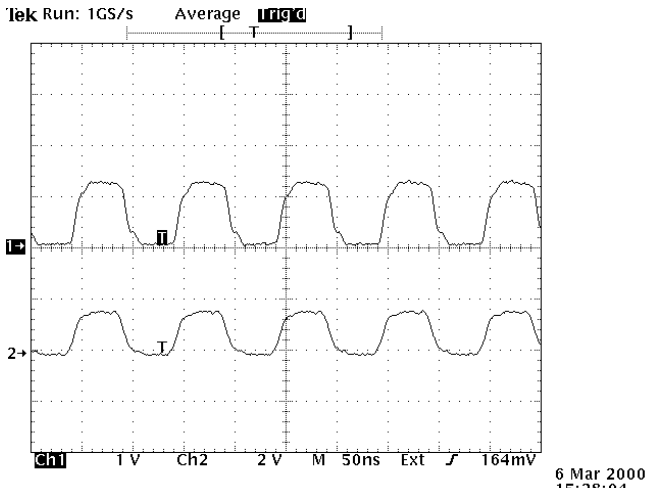
Top: OUT, 0.2A into 6Ω load at end of LZ6 transmission line. 50 ns PW, 10 MHz Internal Trigger mode. 1V/div, 50 ns/div. Bottom: Monitor output, 10 kΩ load. 2V/div, 50 ns/div
