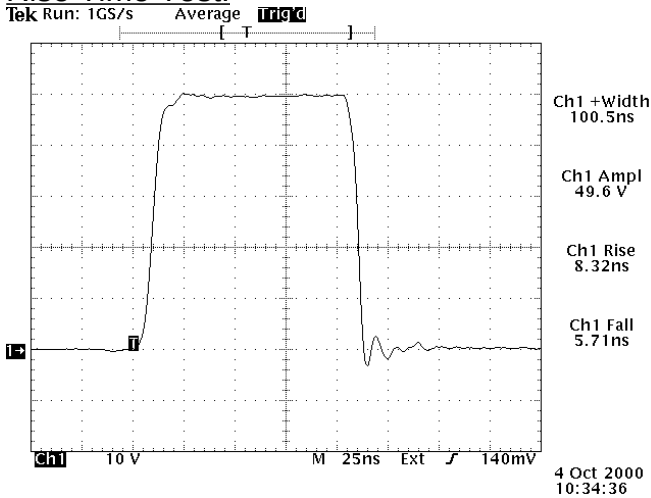
Output waveform (10V/div, 25ns/div) for: PRF=10 kHz, PW=100ns, AMPL=+100V, ZOUT=50Ω
