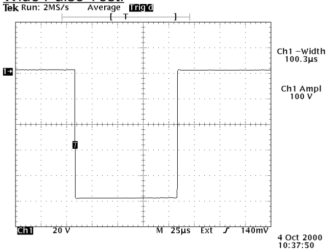
Output waveform (20V/div, 25us/div) for: PRF=100 Hz, PW=100us, AMPL=-100V, ZOUT=2Ω
