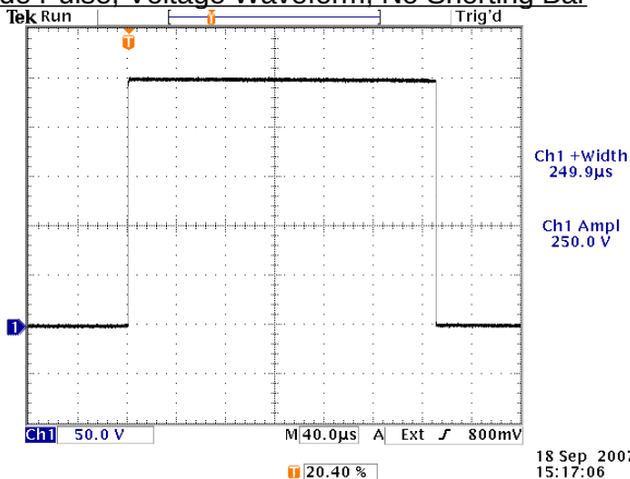
Wide Pulse, Voltage Waveform, No Shorting Bar
