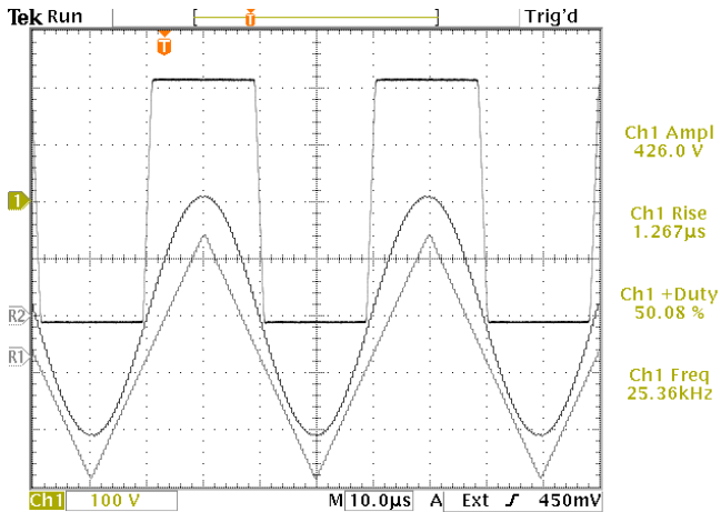
3 Feb 2003 11:46:45 Square, Sine, and Triangle outputs into a 50kΩ load. 25 kHz. 100 V/div, 10 us/div.
