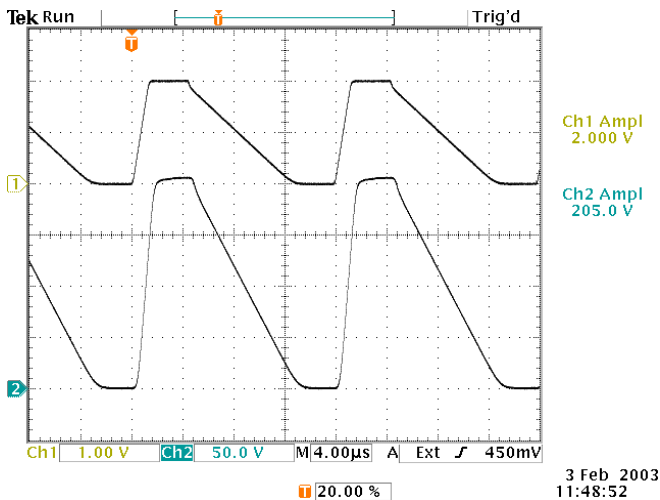
3 Feb 2003 11:48:52 EXT mode, maximum gain. Top: +2V pulse in. 1V/div, 4 us/div. Bottom: +200V pulse out. 50V/div, 4 us/div.
