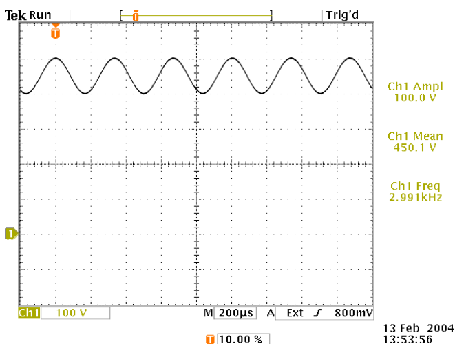
+450V offset with \pm 50V Amplitude, 3 kHz, sine wave 100V / div, 200 us / div.
