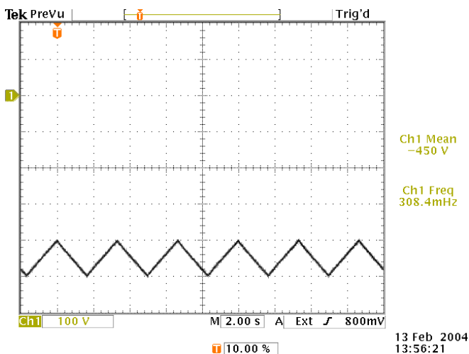
-450V offset with \pm 50V Amplitude, 0.3 Hz, triangle wave 100V / div, 2 sec / div.
