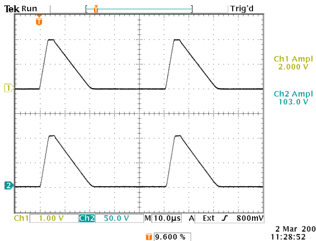
EXT mode, maximum gain. Top: +2V pulse in. 1V/div, 10 us/div. Bottom: +100V pulse out. 50V/div, 10 us/div.
