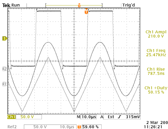
Square, Sine, and Triangle outputs into a 10 kΩ load. 25 kHz. 50 V/div, 10 us/div.
