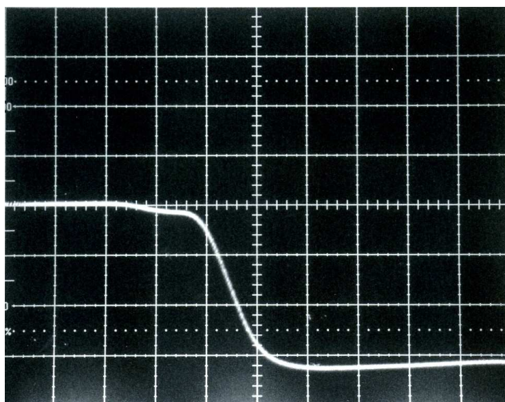
-3V output into 50 Ohms. 1 V/div, 1 ns/div.
