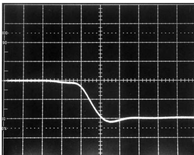
-2V output into 50 Ohms. 1 V/div, 1 ns/div.
