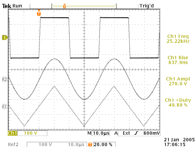
Square, Sine, and Triangle outputs into a 500 Ω load. 25 kHz. 100 V/div, 10 us/div.
