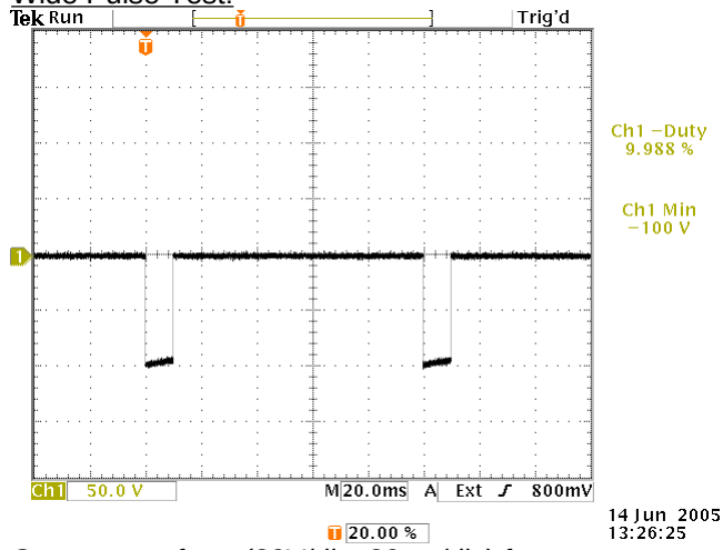
Output waveform (20V/div, 20 us/div) for: PRF=10 Hz, PW=10 ms, AMPL=-100V, ZOUT=2Ω
