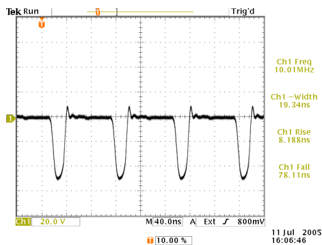
-50V, Z_{OUT}=2\Omega , 50 \Omega load, near minimum PW, 10 MHz
