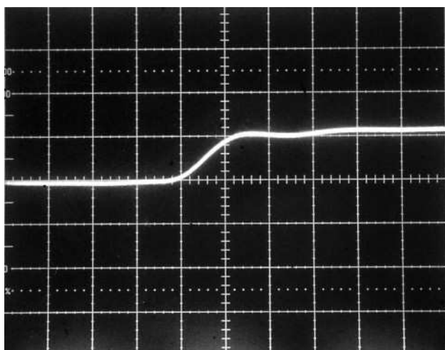
1V output into 50 Ohms. 1 V/div, 1 ns/div.
