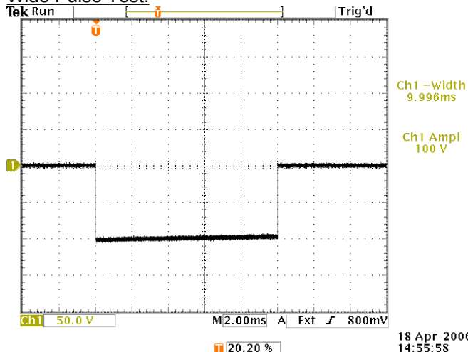
Output waveform (50V/div, 2 ms/div) for: PRF=5 Hz, PW=10 ms, AMPL=-100V, ZOUT=2Ω
