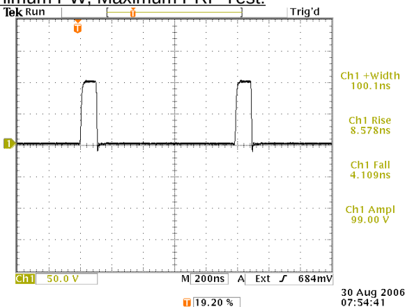
Output waveform (50V/div, 200 ns/div) for: PRF=1 MHz, PW=100 ns, AMPL=MAX, ZOUT=2Ω
