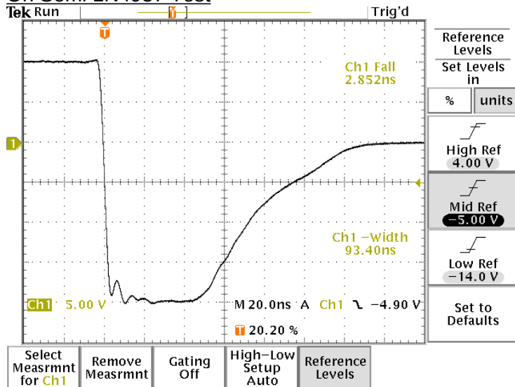
On Semi 1N4937 Test
