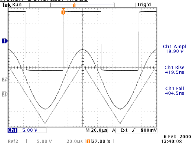
Square, Sine, and Triangle outputs into a 9 Ω load. 10 kHz. 5 V/div, 20 us/div.
