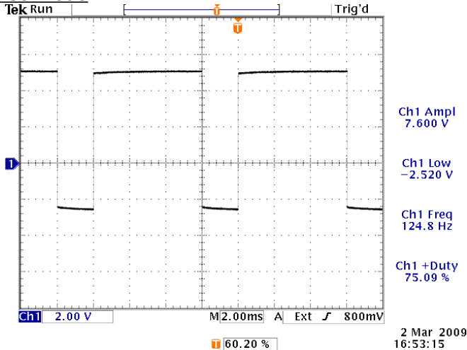
+7.5V pulse at 125 Hz, with -2.5V offset and 75% duty cycle. 2 V/div, 4 ms/div.
