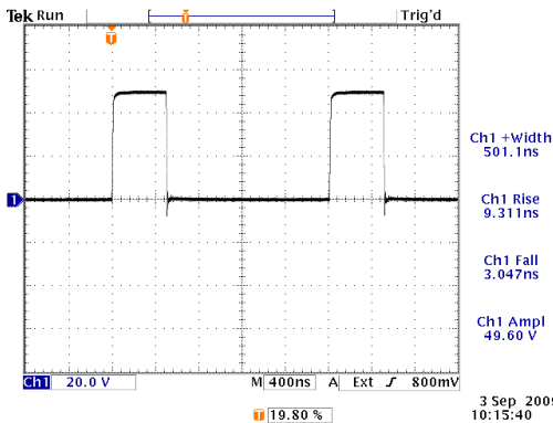
+50V, Z_{OUT}=2\Omega , 50 \Omega load, PW = 500 ns, 500 kHz
