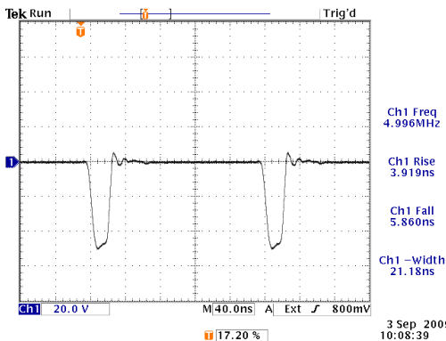
-50V, Z_{OUT}=2\Omega , 50 \Omega load, PW = 20 ns, 5 MHz
