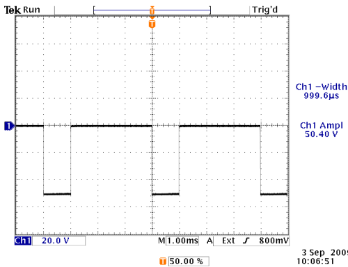
-50V, Z_{OUT}=2\Omega , 50 \Omega load, PW = 1 ms, 250 Hz
