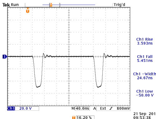
-50V, ZOUT=2Ω, 50Ω load, PW = 25 ns, 5 MHz
