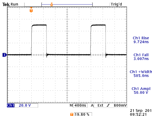
+50V, ZOUT=2Ω, 50Ω load, PW = 500 ns, 500 kHz
