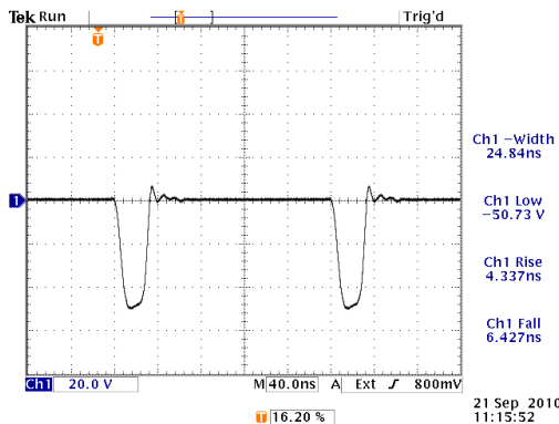
-50V, Z OUT =2Ω, 50Ω load, PW = 25 ns, 5 MHz
