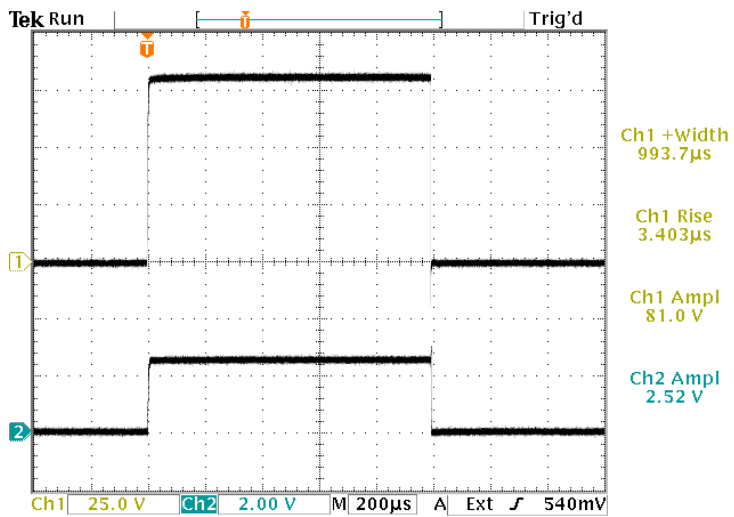
Top: 280 Hz, 1 ms, +12.5A into a 6.54Ω load. 25V/div. Bot: Monitor output (1V / 5A). 200 us/div.
