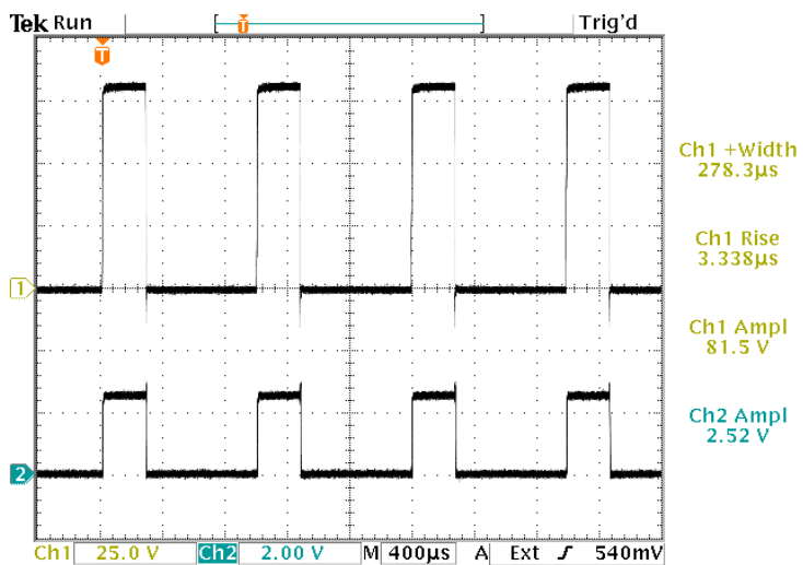
Top: 1 kHz, 280 us, +12.5A into a 6.54Ω load. 25V/div. Bot: Monitor output (1V / 5A). 400 us/div.
