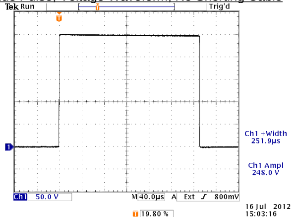
Wide Pulse, Voltage Waveform, No Shorting Cable
