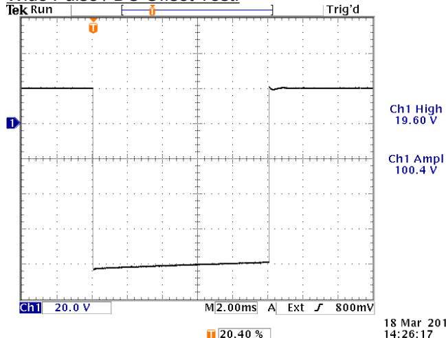
Output waveform (20V/div, 2 ms/div) for: PRF=5 Hz, PW=10 ms, AMPL=MIN, ZOUT=2Ω, with +20V offset
