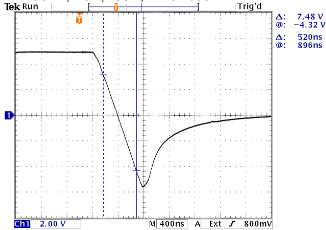
1N4004A, +5A, -80V, < 20 A/us.
