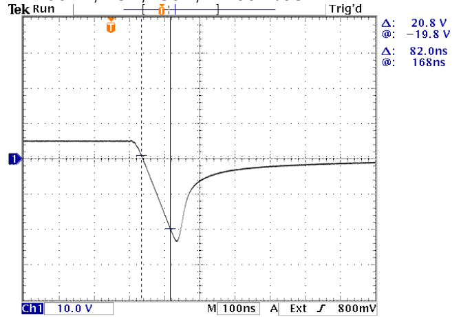
1N4004A, +5A, -80V, > 200 A/us.
