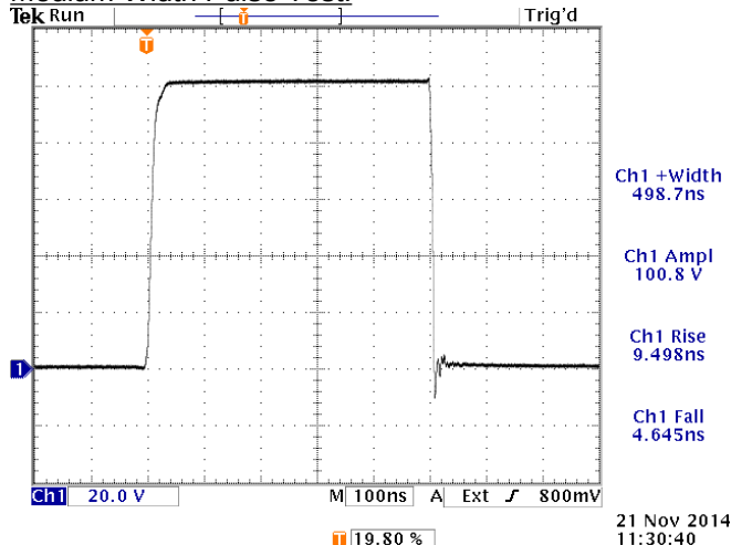
Output waveform (20V/div, 100 ns/div) for: PRF=10 kHz, PW=500ns, AMPL=+100V, ZOUT=2Ω
