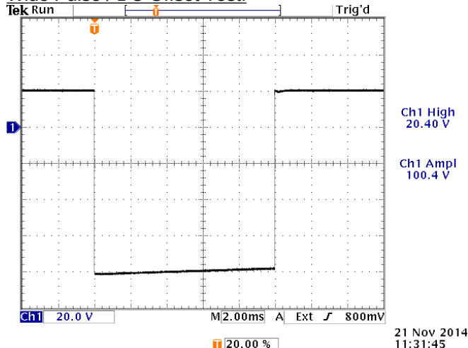
Output waveform (20V/div, 2 ms/div) for: PRF=5 Hz, PW=10 ms, AMPL=-100V, ZOUT=2Ω, with +20V offset
