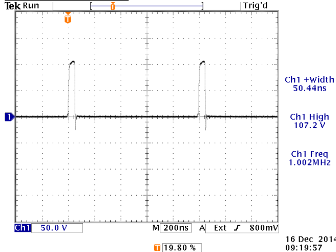
Output waveform (50V/div, 200 ns/div) for: PRF=1 MHz, PW=50 ns, AMPL > +100V, ZOUT=2Ω
