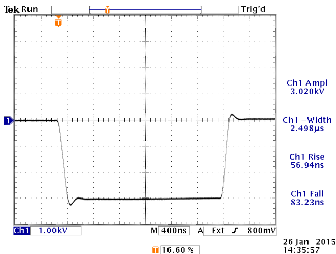
1 kHz, 2.5 us, -3000V into a 10 kΩ load. 1000 V/div, 400 ns/div.
