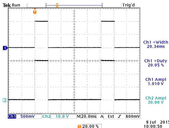
Top: +1V pulse in. 500 mV/div, 20 ms/div. Bottom: +30V out, into 20Ω (+1.5A). 10 V/div.
