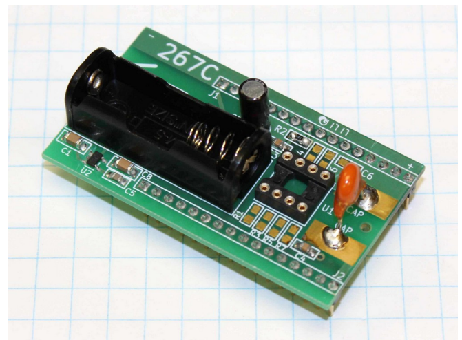
150 pF capacitor (orange) on daughterboard
